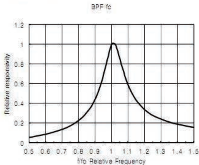
[ Fig.8 ] BPF Fc Curve
