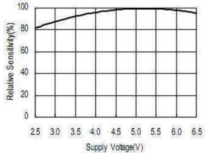
[ Fig.5 ] Sensitivity vs. Supply Voltage
