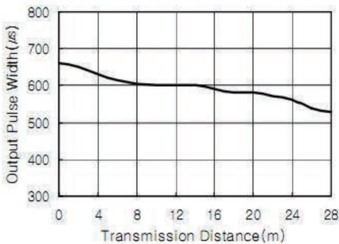
[ Fig.6 ] Output Pulse Width vs. Distance
