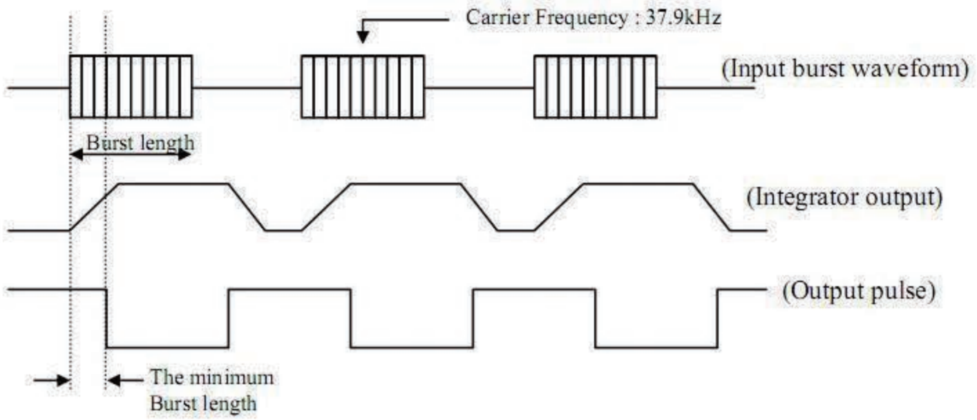
[ Fig. 1 ] Data Signal diagram
