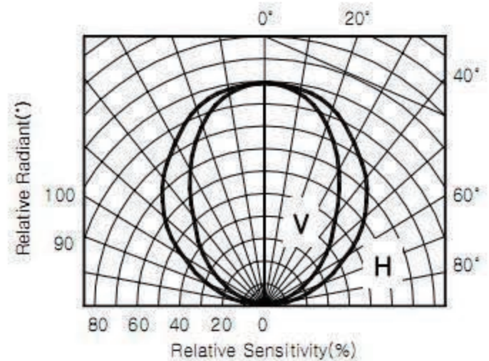
[ Fig.7 ] Directivity (Horizontal)
